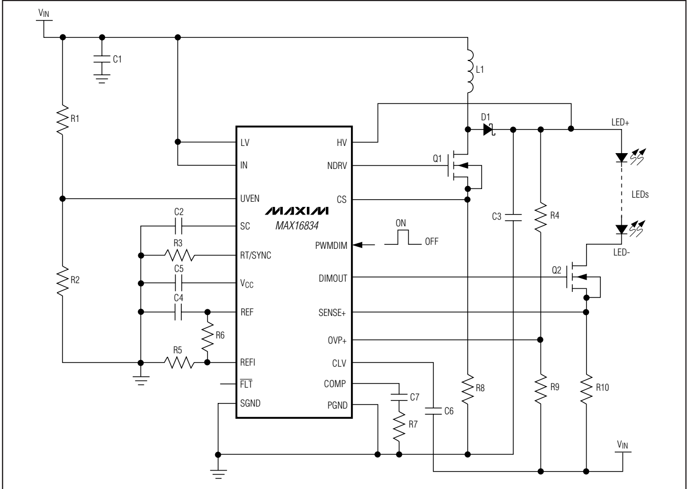
Figure 3. Buck-Boost LED Driver ( V_{LED+} < 28V )
